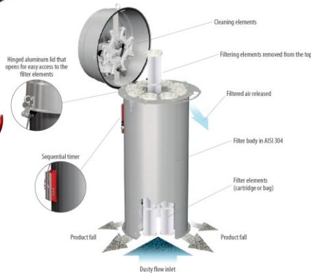
Silo Vent Filter
