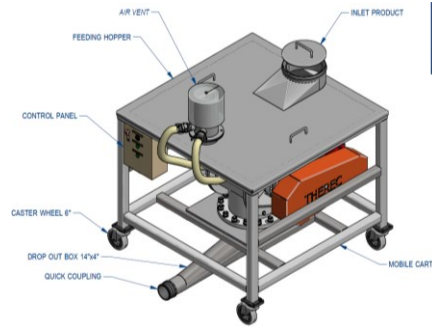
Mobile Air-Lock Rotary valve
