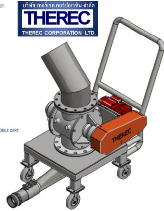
Mobile Air-Lock Rotary valve
