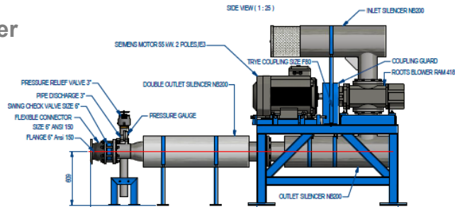
Roots Blower Package
